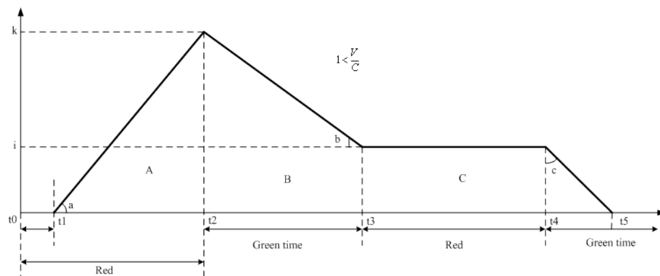
Figure 5 - Case 1- no initial queue for the observed group
