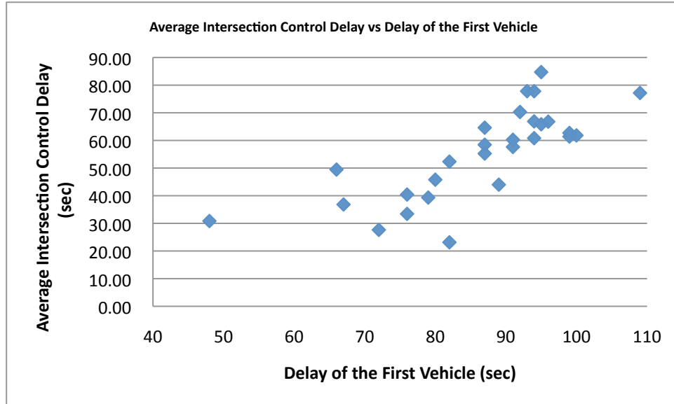
Figure 2 - Average Intersection Control Delay vs Delay of the First Vehicle in the observed group
