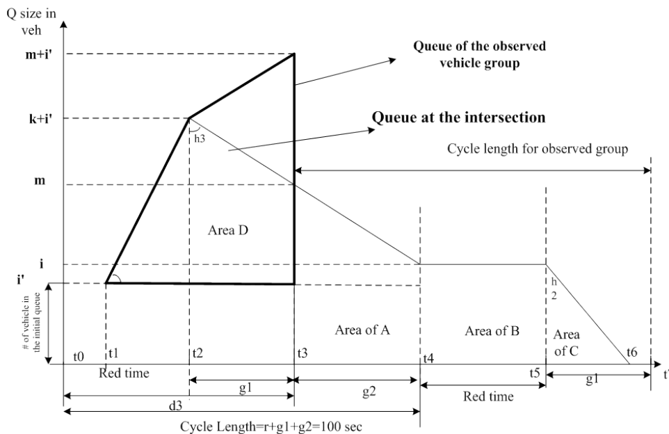
Figure 6 - Case 2- d_3 is smaller than a Cycle Length
