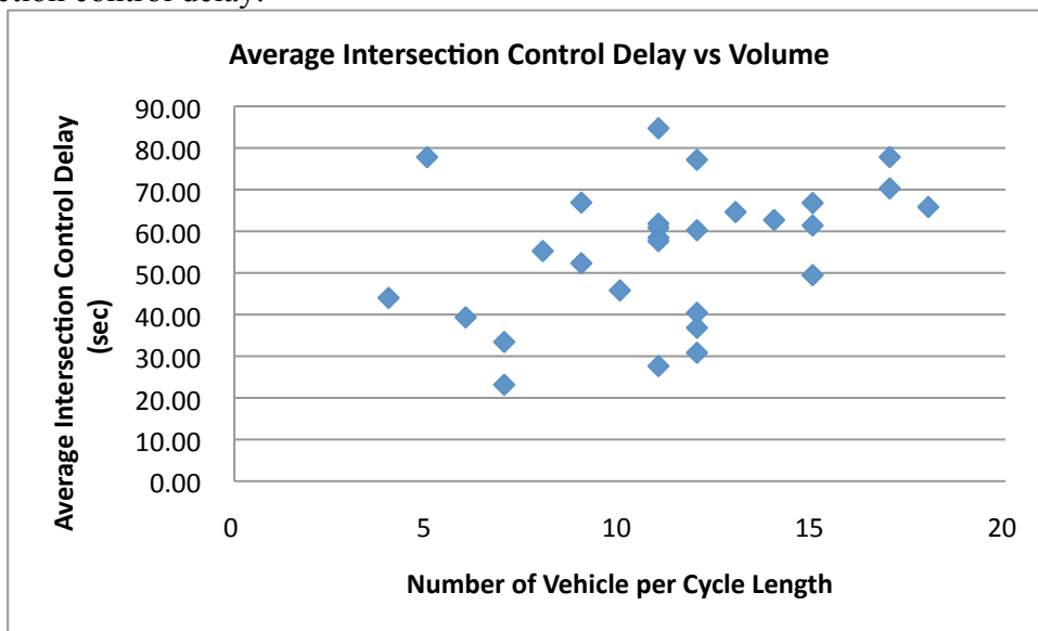
Figure 1 – Average Intersection Control Delay vs Volume
