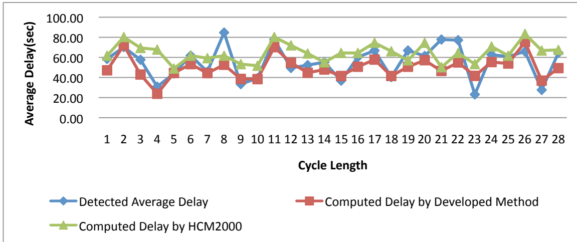
Figure 8- Detected Average Delay and Computed Delay with HCM2000 vs Computed Delay with Developed Method
